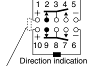
2-coil latching
